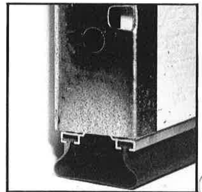
"U" Shaped Bottom Vinyl Weatherstripping
