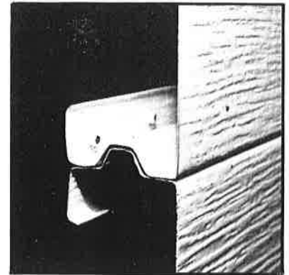
Roll Formed Steel Tongue & Groove Section Joints
